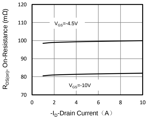
Figure 3. Drain-Source On-Resistance
